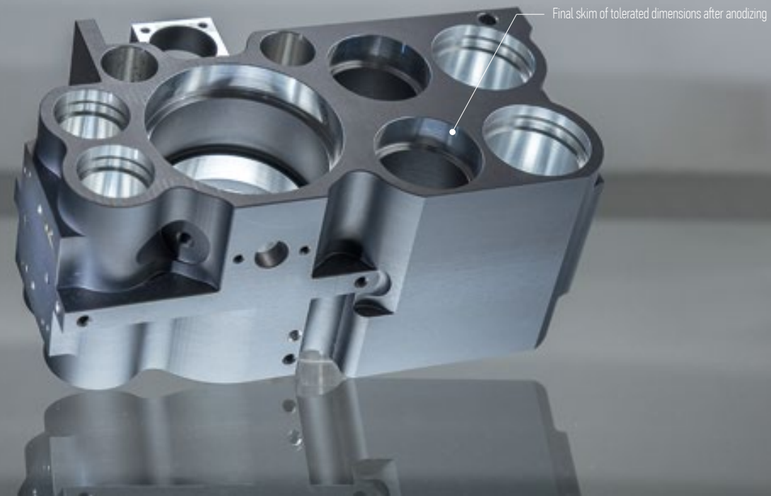
Final skim of tolerated dimensions after anodizing
